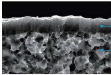
硬度高, 光滑涂层, 润滑剂层 High hardness, smooth coating, Lubricant layer 坚韧的基材/Tough substrate
