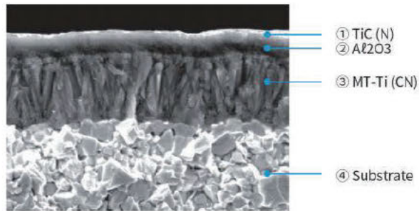
CVD涂层横截面图 Cross-sectional view of CVD coating
